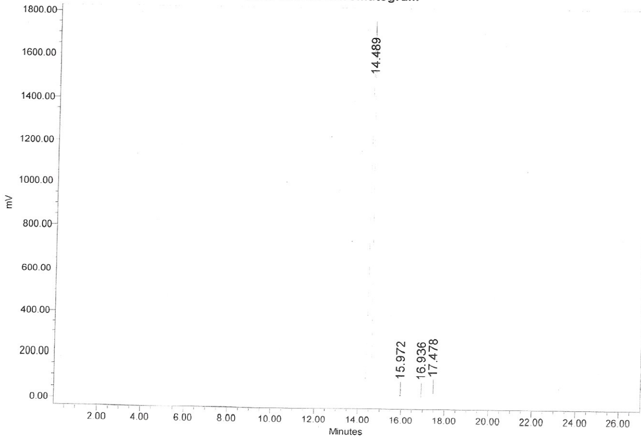
Auto-Scaled Chromatogram
